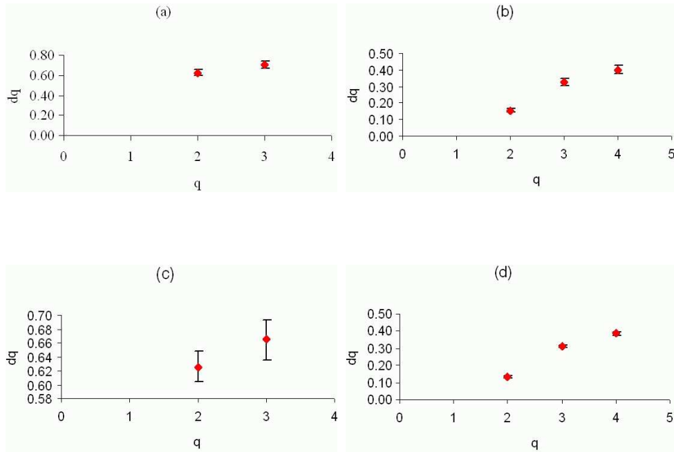
Fig. 1. Variation of the anomalous fractal dimension with the order of the moment for a) K^- - \text{CNO} , b) K^- - \text{AgBr} , c) p - \text{CNO} and d) p - \text{AgBr} interactions.
