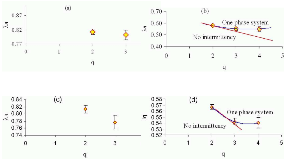
Fig. 2. Variation of \lambda_q against q for a) K^- - CNO, b) K^- - AgBr, c) p - CNO and d) p - AgBr interactions.
