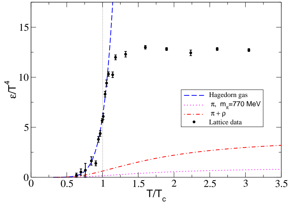
Fig. 1. Energy density of lattice QCD (circles) and Hagedorn gas (long dashed line) as functions of the reduced temperature T/T_c . The contributions of pion gas (dotted line) and gas of pions and \rho mesons (dash-dotted line) are shown for a comparison. Note that the pion mass on the lattice is not the physical one.
