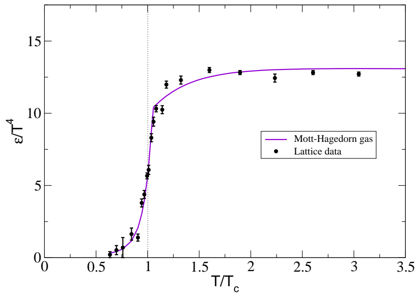
Fig. 2. Fit of the lattice QCD data [1] with the Mott–Hagedorn resonance gas model (6). For details see text.
