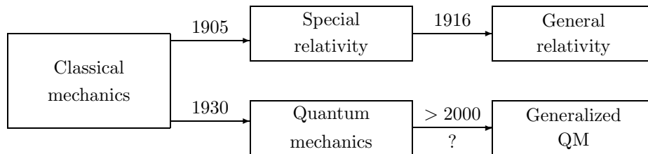
Figure 1. The Generalizations of classical mechanics.
