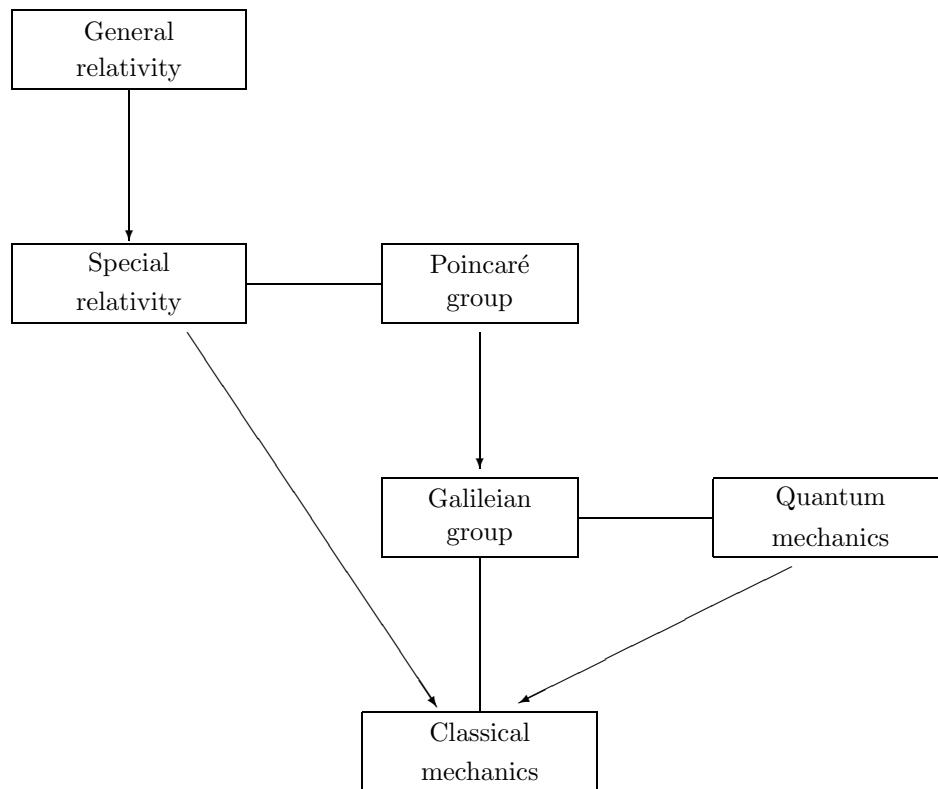
Figure 2. The Current structure of physics.
