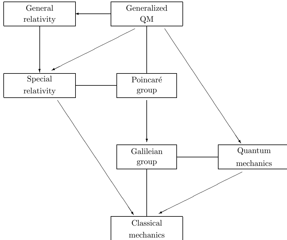
Figure 3. A new hypothetical model of physics.
