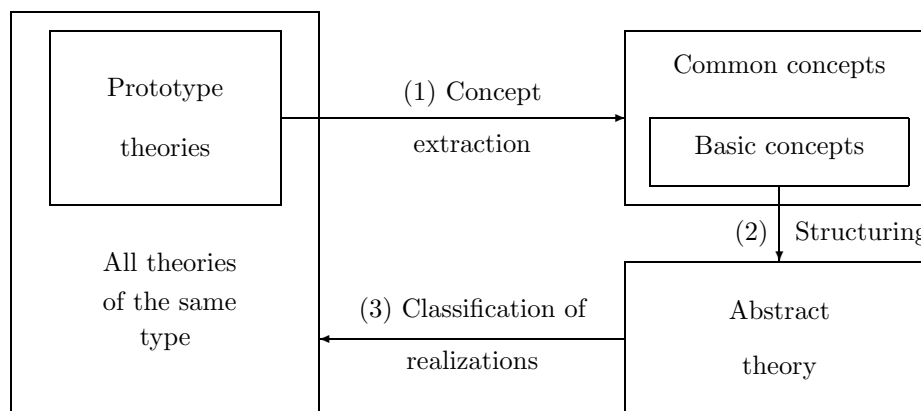
Figure 4. The generalization procedures
